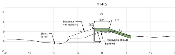
SNIT E-E, 1:150
