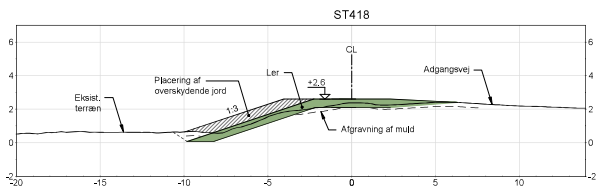
SNIT F-F, 1:150
